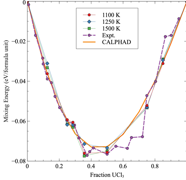
Figure 9: Mixing energies for NaCl- \text{UCl}_3 at 1100, 1250 and 1500 K. Pure NaCl and \text{UCl}_3 are used as references. The calculated results are compared to experiments [5] and a thermodynamic assessment [7].
