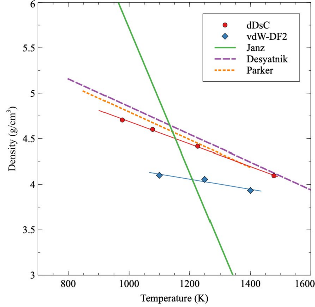
Figure 5: Density of \text{UCl}_3 predicted the DFT-dDsC model for the dispersion forces (small cell with 64 atoms). Experimental data is represented by the correlations plotted as purple dashed [3], green solid [2] and orange dotted lines [4]. The lines following the calculated data points were obtained as least-squares fits, the equations of which are summarized in Table 1.
