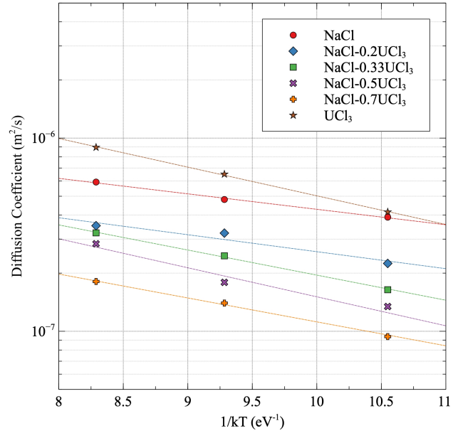
Figure 12: Arrhenius diffusion of NaCl-UCl 3
