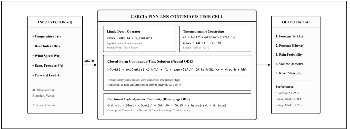
Fig. 2. Internal mathematical architecture of the Garcia PINN-LNN Cell. Combines closed-form liquid exponential decay, Magnus-Tetens saturation bounds, Lifted Condensation Level (LCL) convective depth activation, and catchment hydrodynamic continuity.
