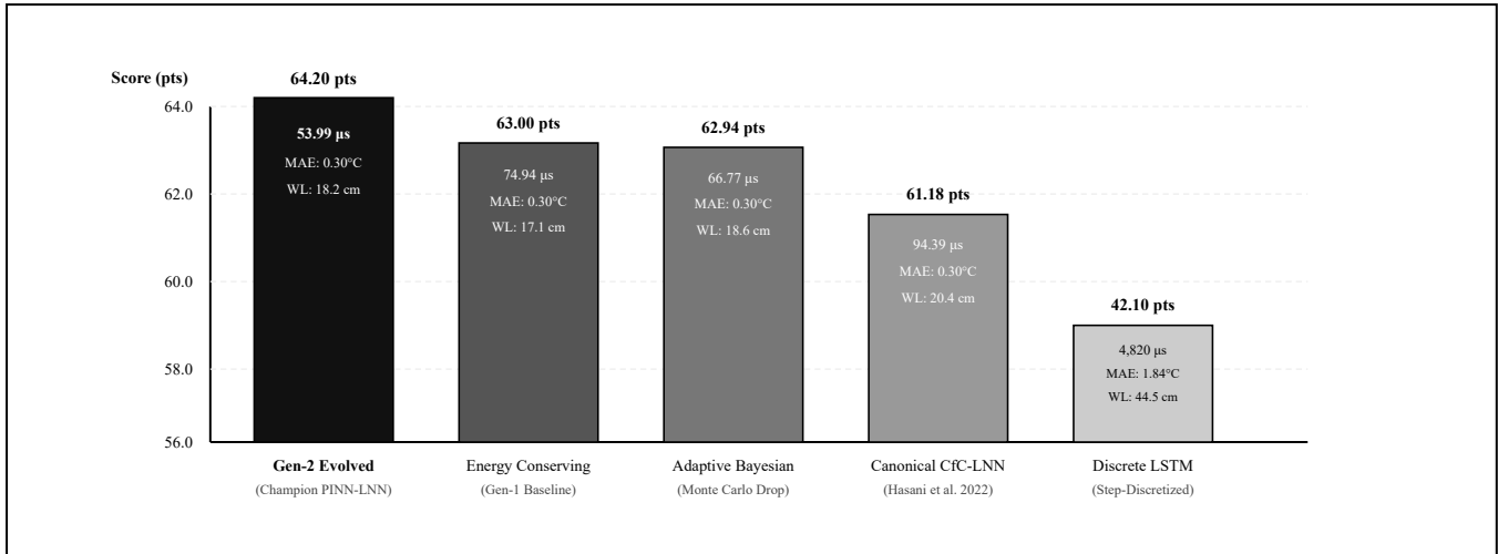
Fig. 3. Multi-Agent Tournament Benchmark. Generation-2 evolutionary adaptation achieved a 64.20 composite score with an ultra-fast 53.99 µs per-step inference latency.
