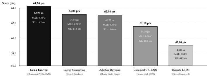
Fig. 3. Multi-Agent Tournament Benchmark. Generation-2 evolutionary adaptation achieved a 64.20 composite score with an ultra-fast 53.99 \mu s per-step inference latency.
