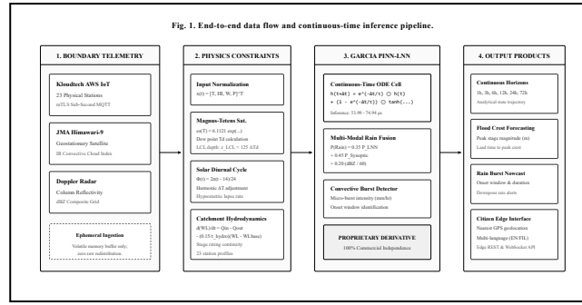
Fig. 1. End-to-end data flow and continuous-time inference pipeline. Boundary telemetry is ingested ephemerally into volatile memory as initial conditions; the Garcia PINN-LNN continuous engine computes latent ODE trajectories; only original computed derivatives are exposed to user interfaces.
