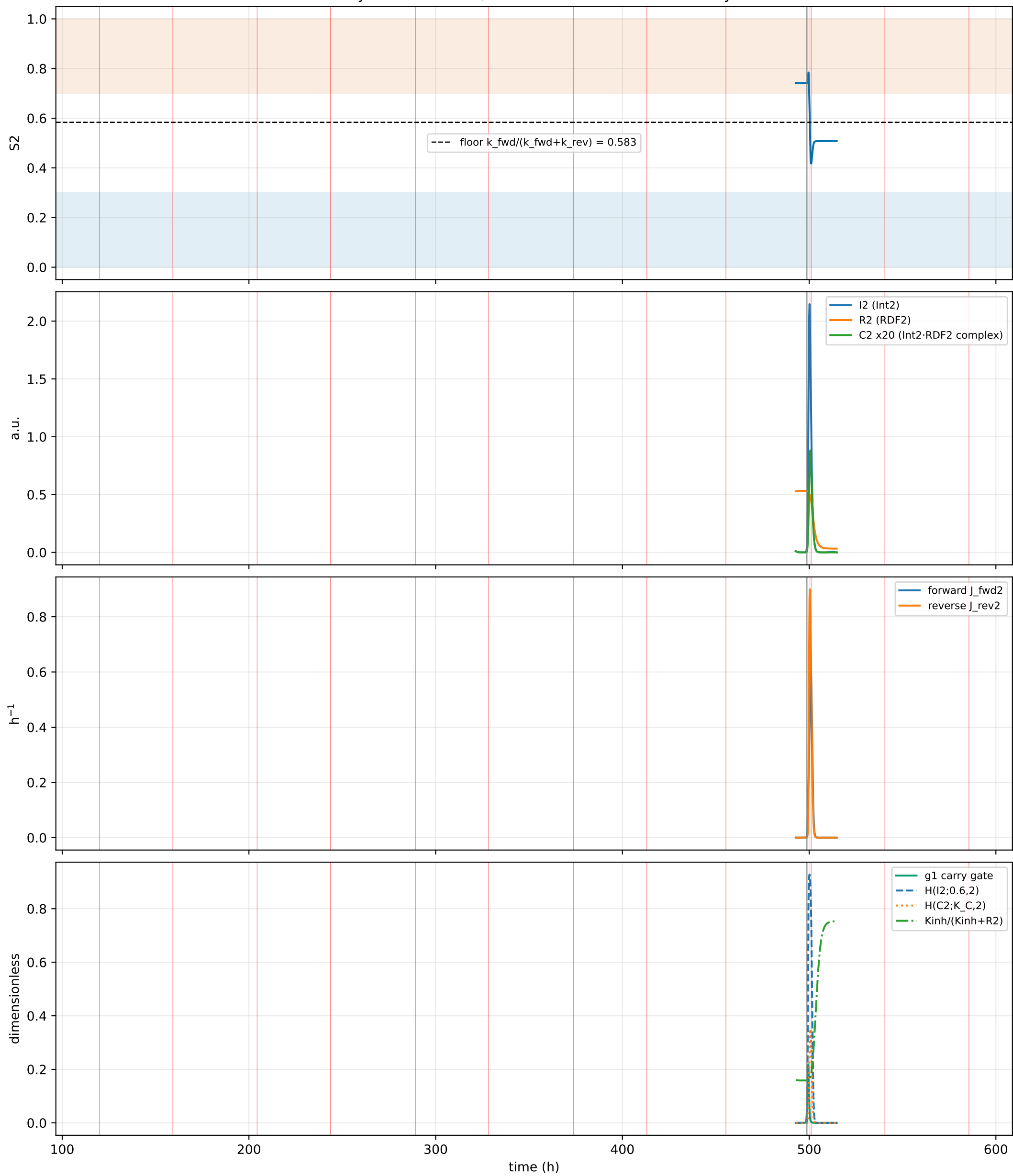
bit2 at carry1 mRNA 4 min / maturation 60 min — one carry window
