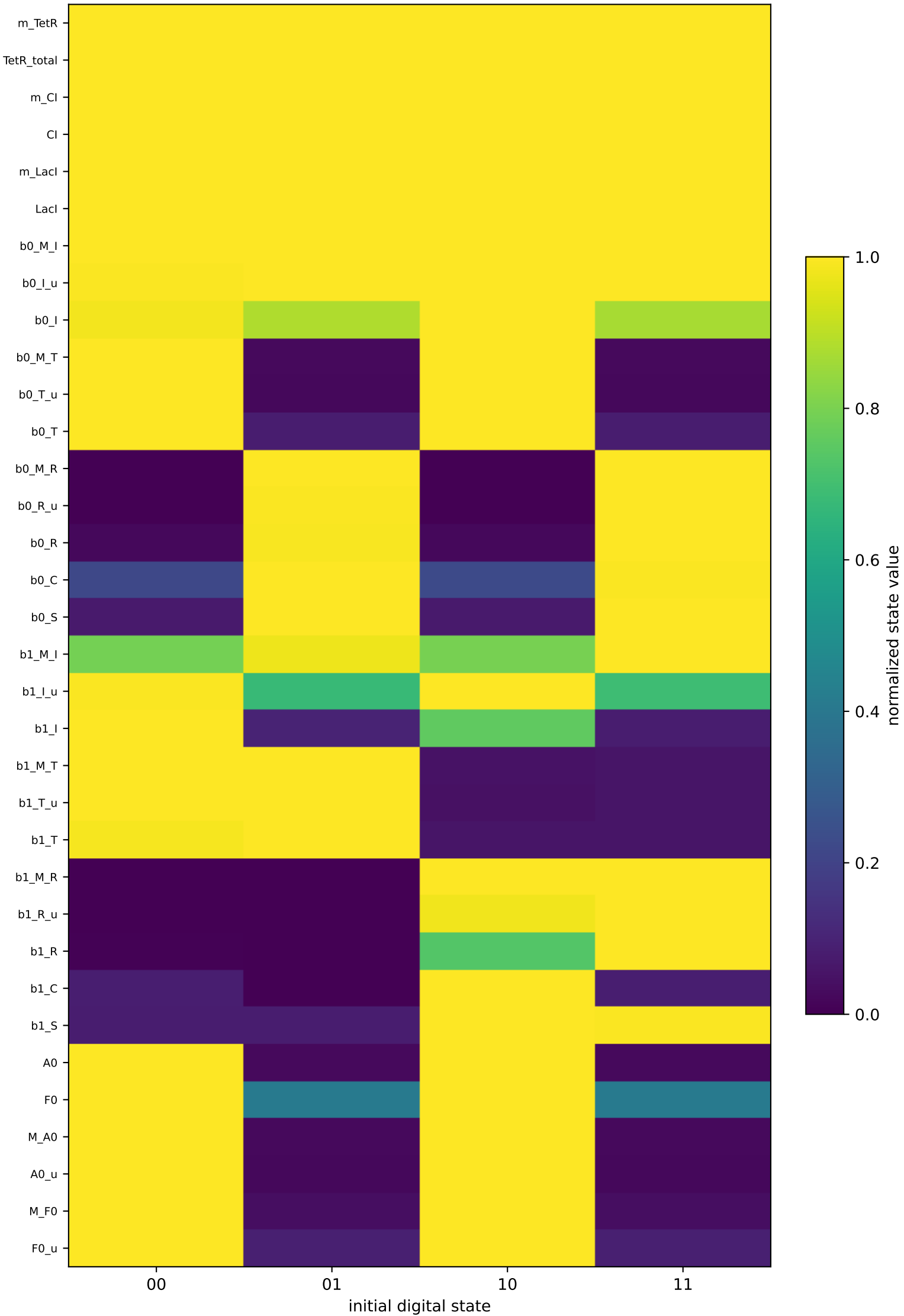
Self-consistent 34-state initial conditions (each molecular state normalized across four branches)
