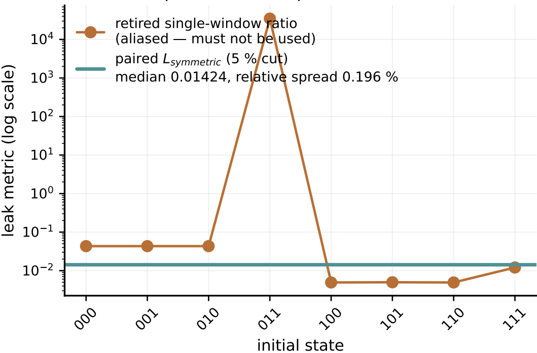
(B) The retired metric spans 3.5 \times 10^4 for one and the same circuit; the paired metric spans 0.196 %
