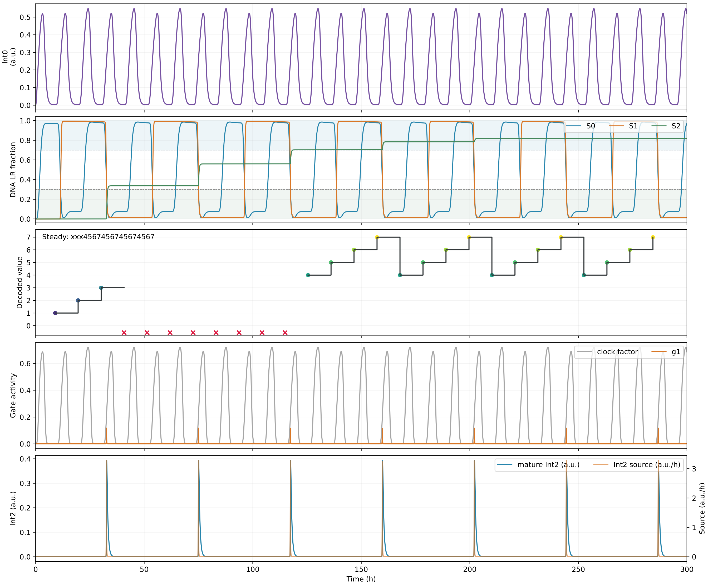
A1 negative autoregulation OFF Han input; 23-state HBY-ZMH-ZMH; diagnostic, not inherited certification
