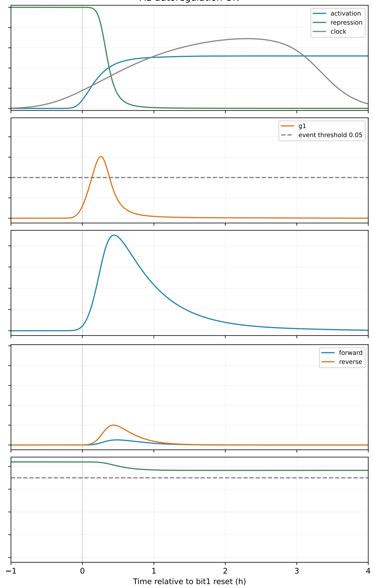
One matched bit1 reset at t=244.364 h; narrow gate pulses and incomplete bit2 writing
