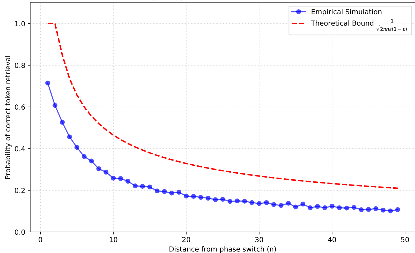
Memory decay of correct token (N=50, \epsilon=0.08 )
