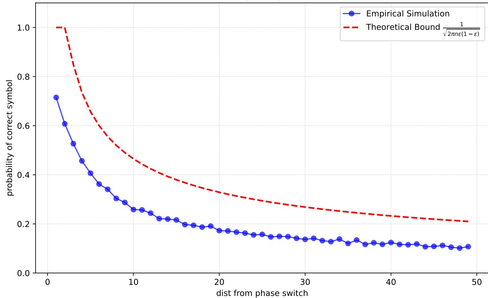
soft stack memory decay (N=50, \varepsilon=0.08 )
