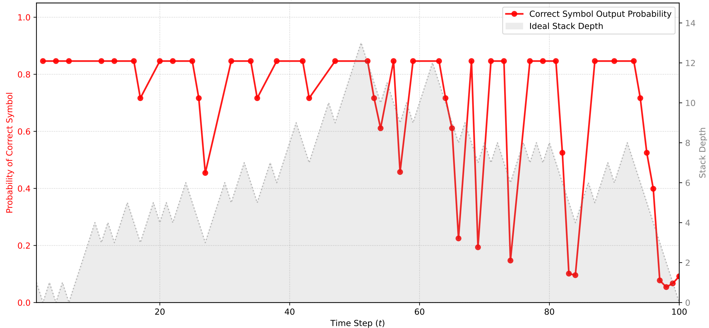
Dyck-1 Memory Fidelity: Interleaved Continuous Stack ( N=100 , \varepsilon=0.08 )
