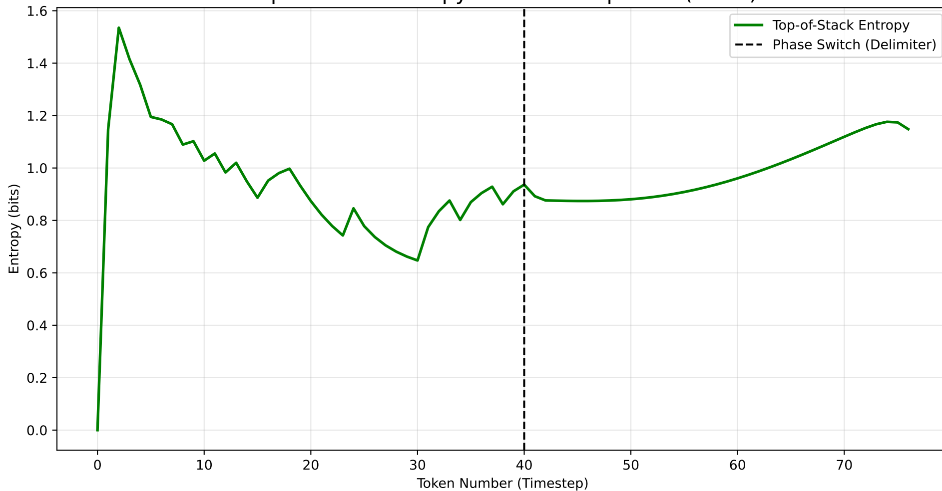
Top-of-Stack Entropy over Full Sequence (L=40)
