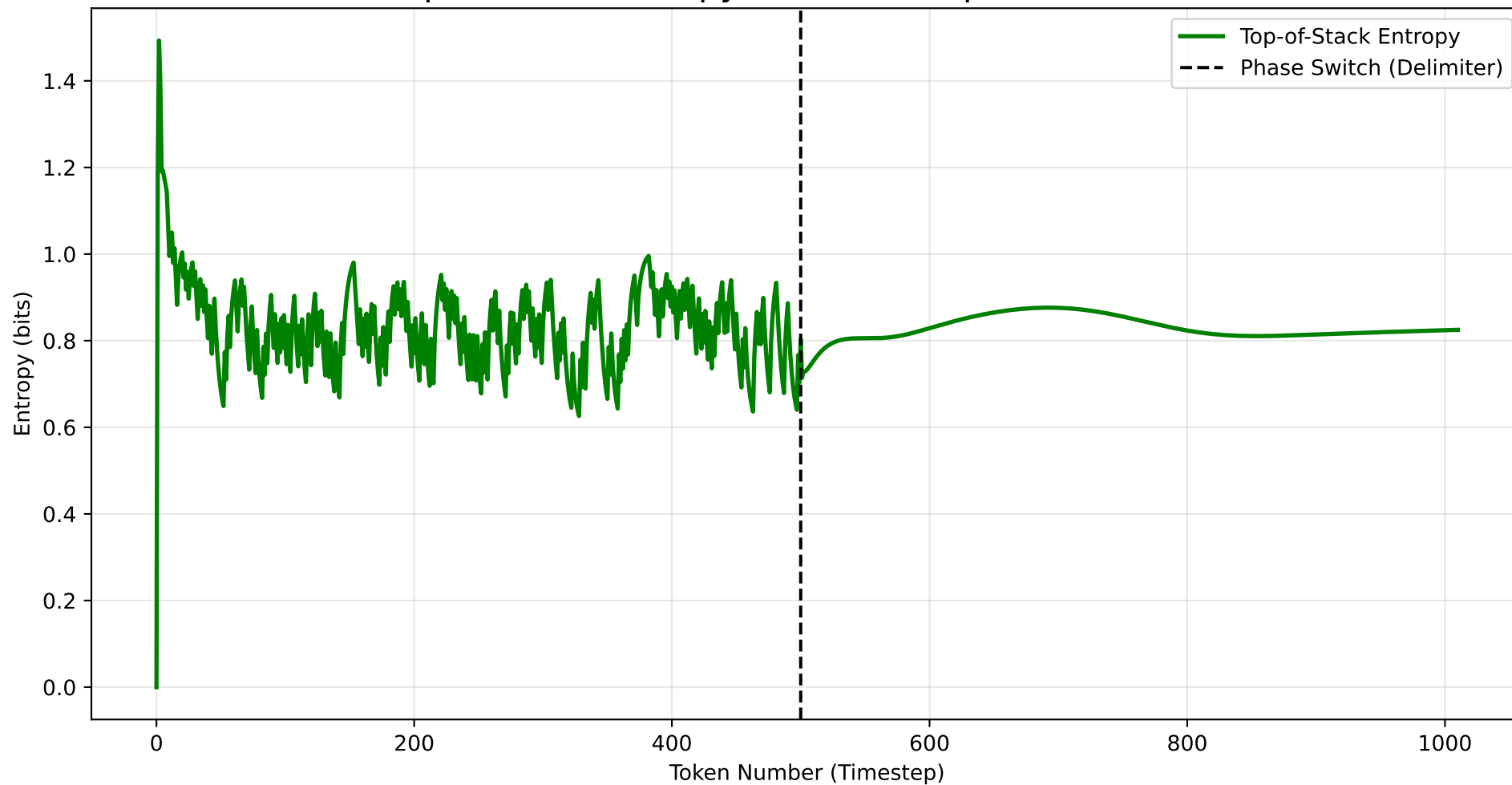
Top-of-Stack Entropy over Full Sequence (L=500)
