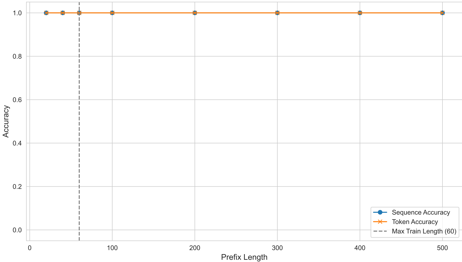
OOD Generalization (Hard Stack Inference)
