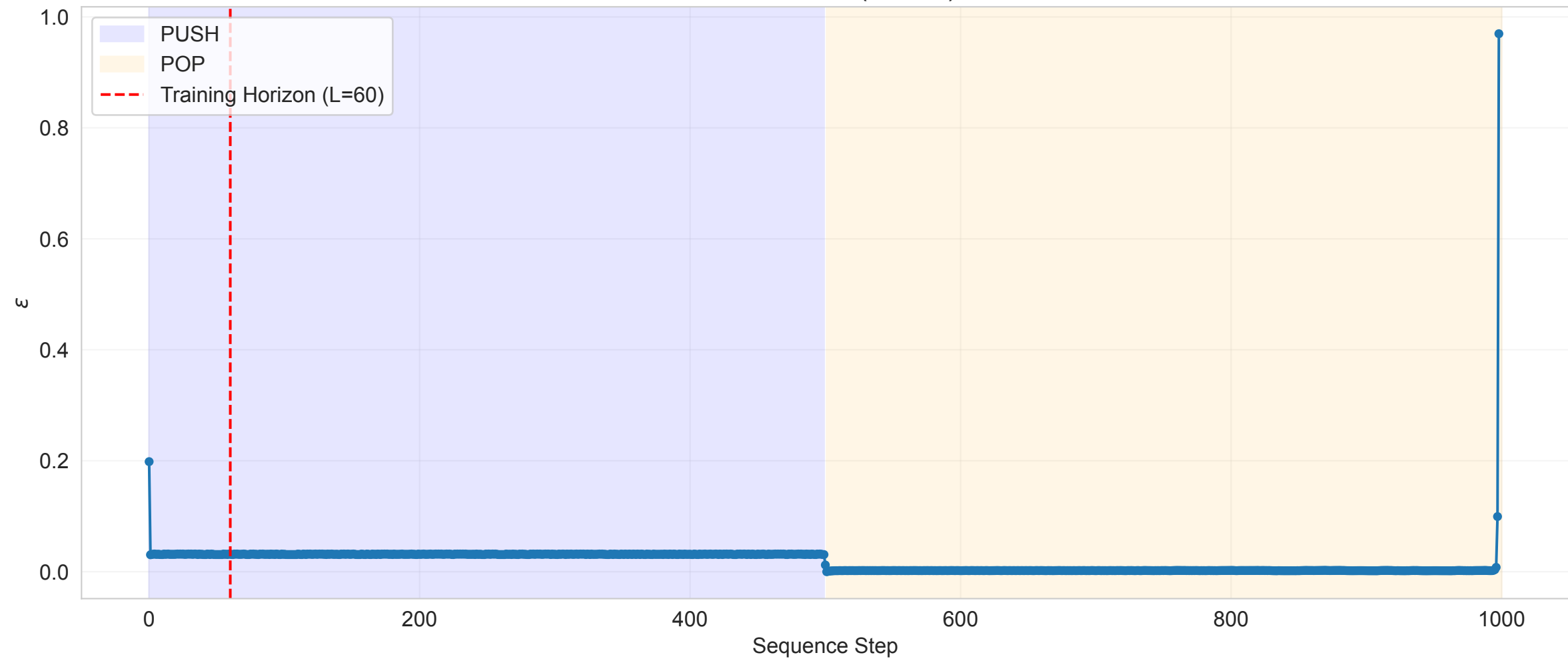
\varepsilon_t over Time (L=500)
