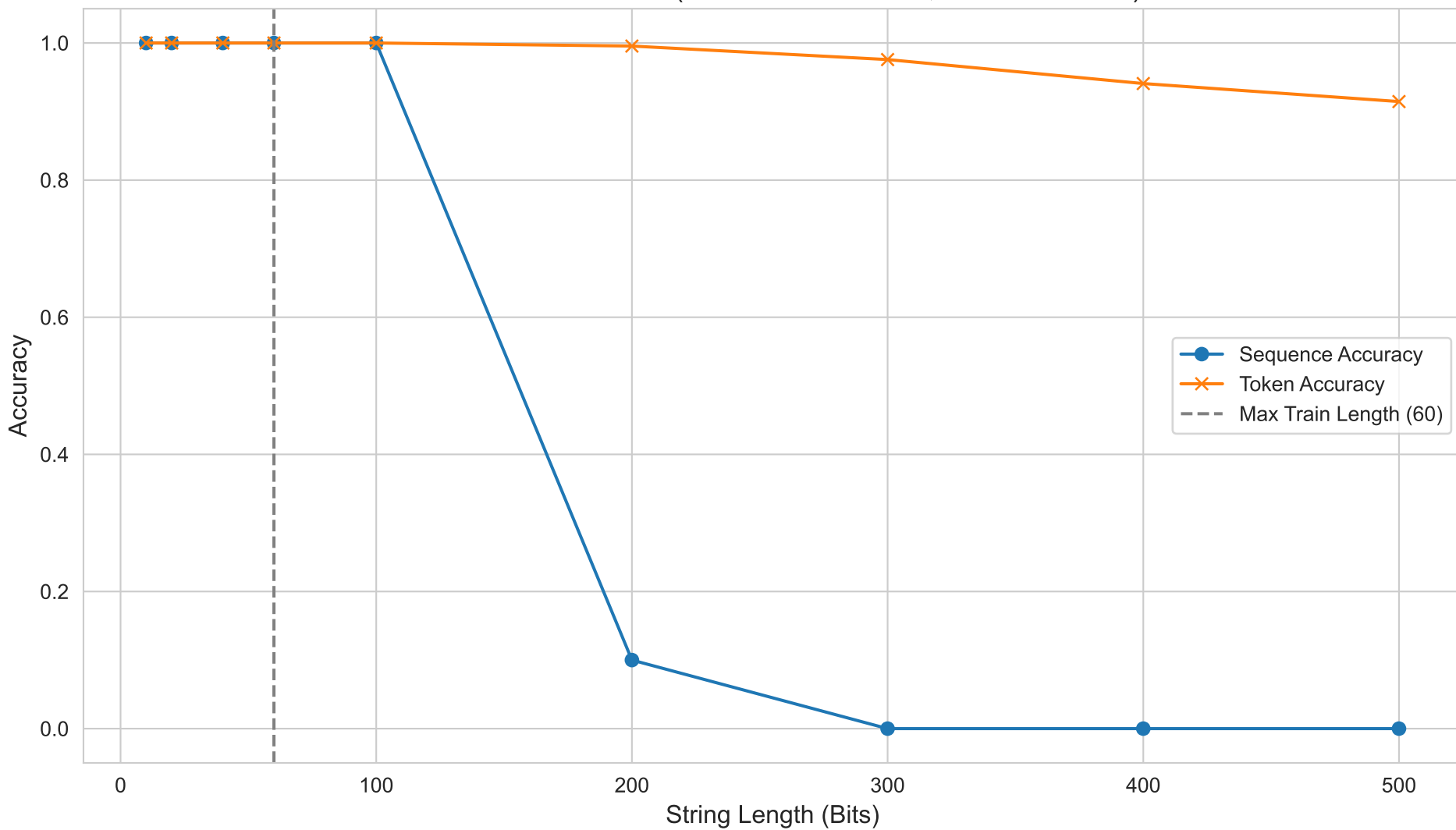
OOD Generalization (64D Softmax State, tanh activation)
