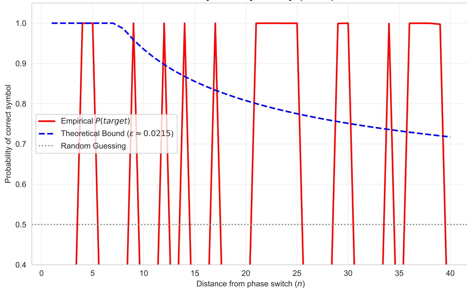
Memory Fidelity Decay (L=40)
