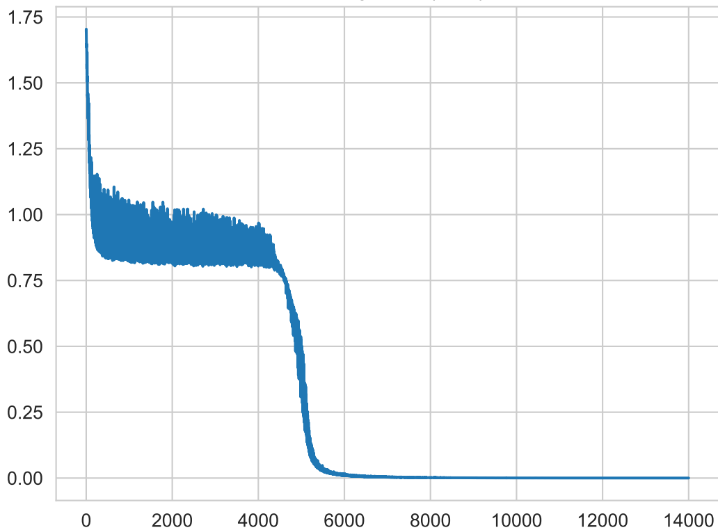
Training Loss (Q=2)
