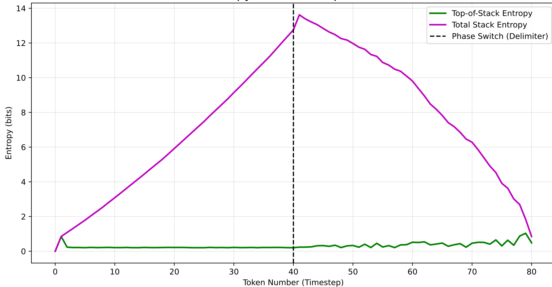
Stack Entropy over Full Sequence (L=40)
