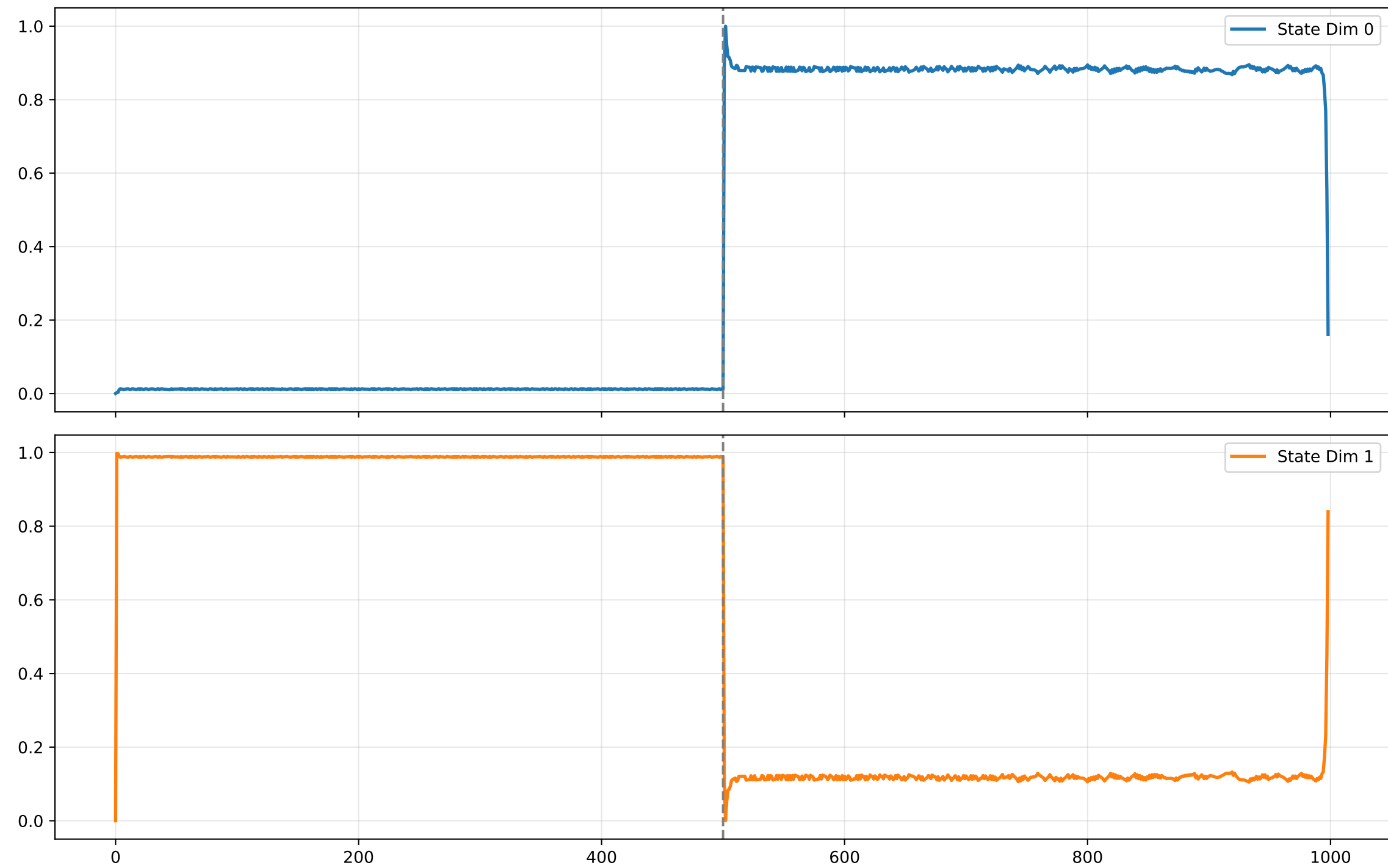
Controller State Components over Time
