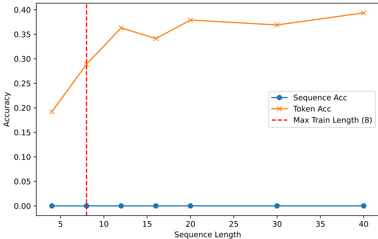
OOD Generalization (Extreme Shortcut)
