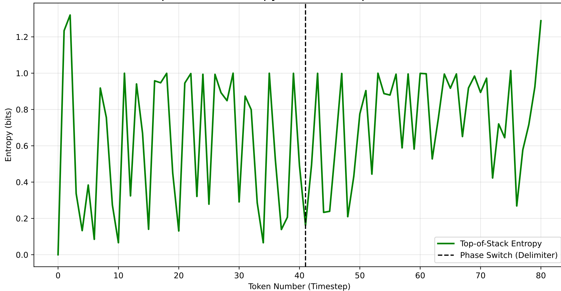
Top-of-Stack Entropy over Full Sequence (L=41)
