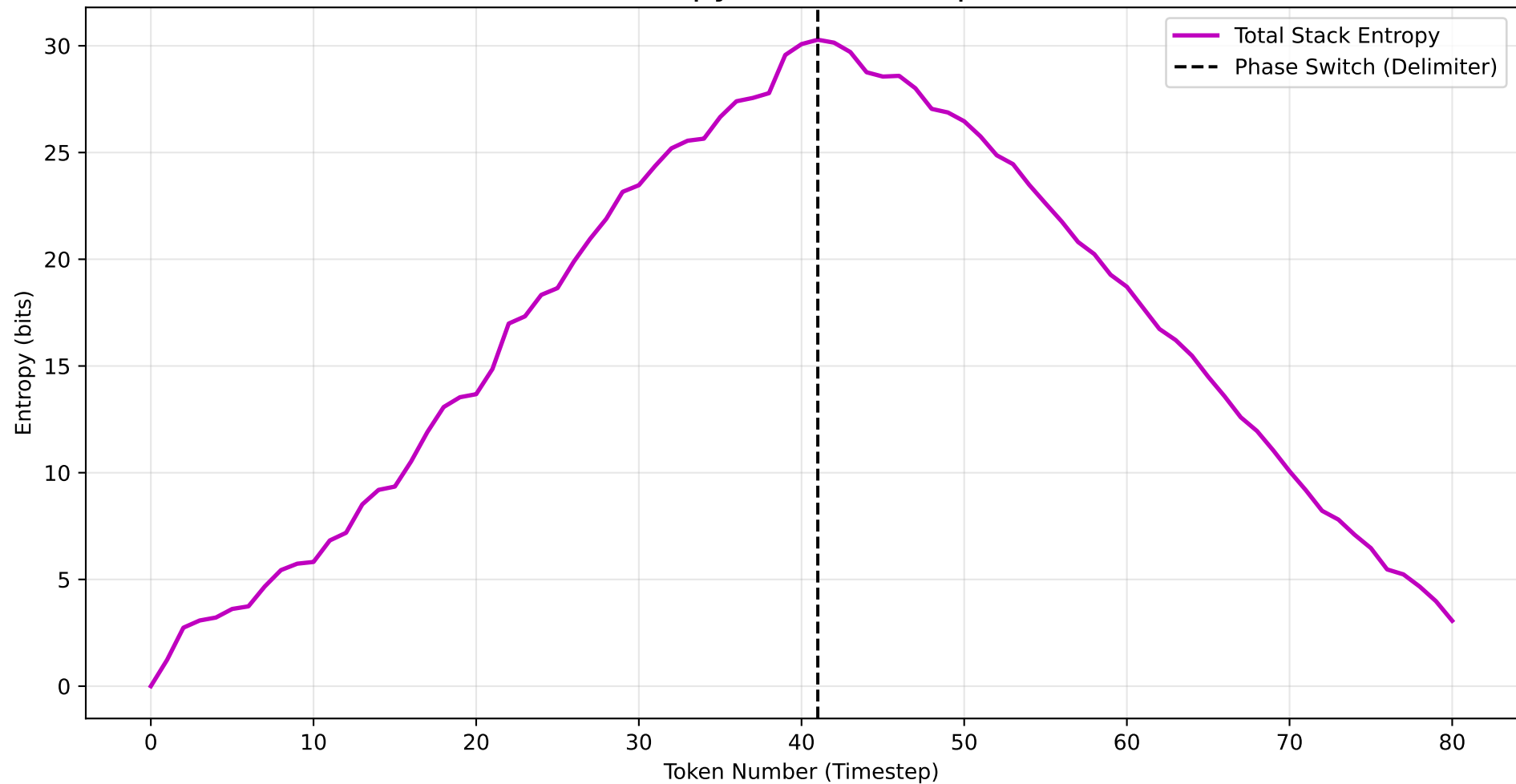
Total Stack Entropy over Full Sequence (L=41)
