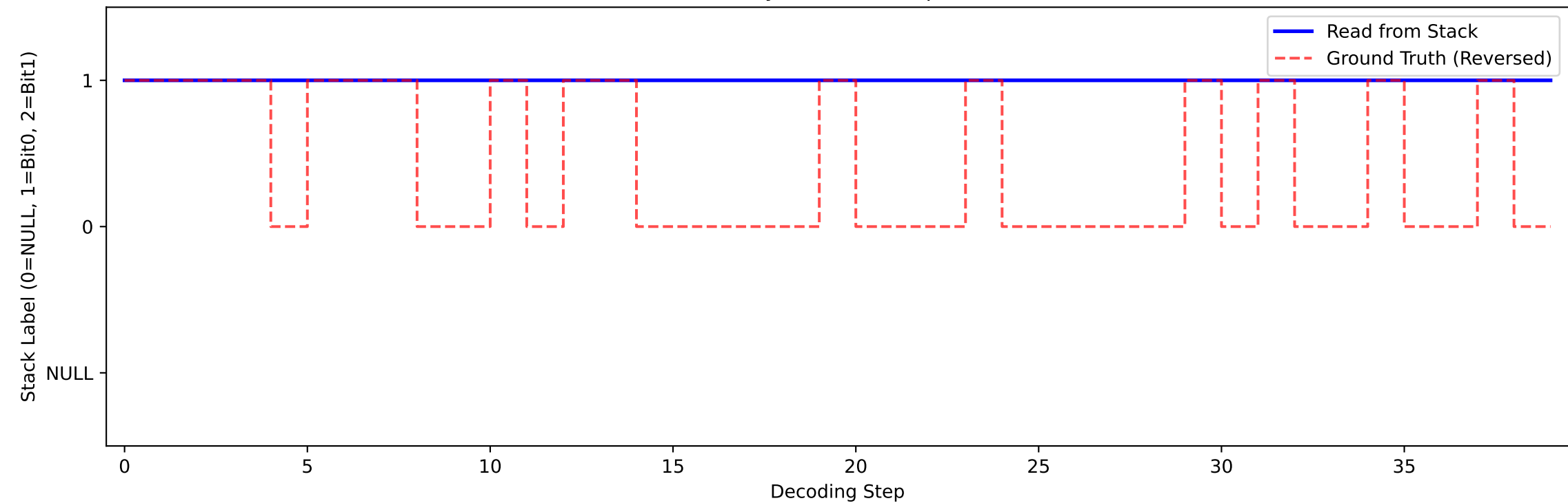
Read Fidelity: Actual vs Expected Bit
