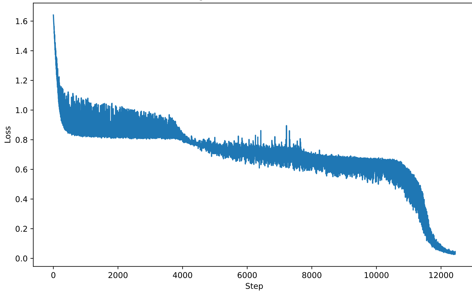
Training Loss Curve (Shortcut Model)
