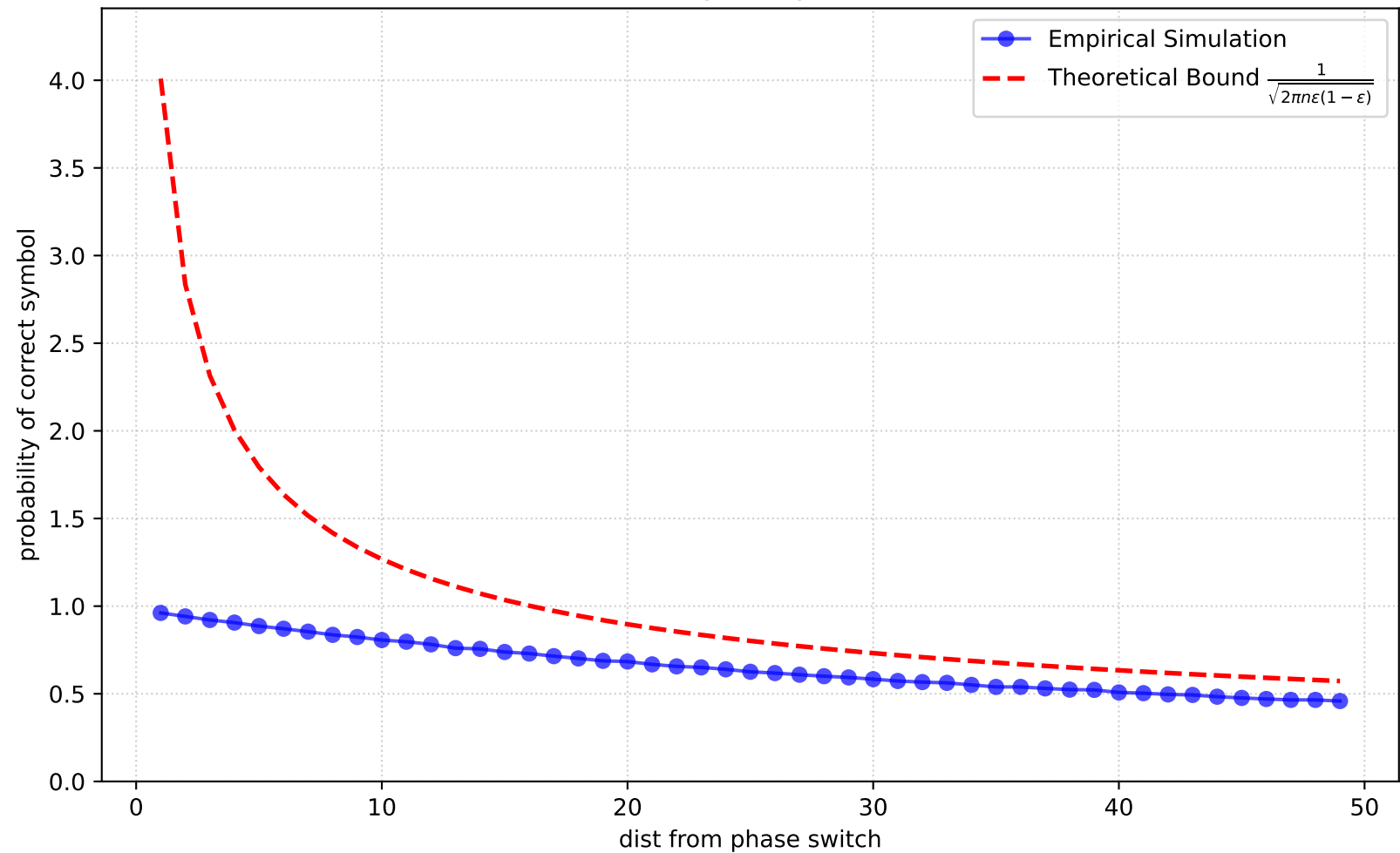
soft stack memory decay (N=50, \varepsilon=0.01 )
