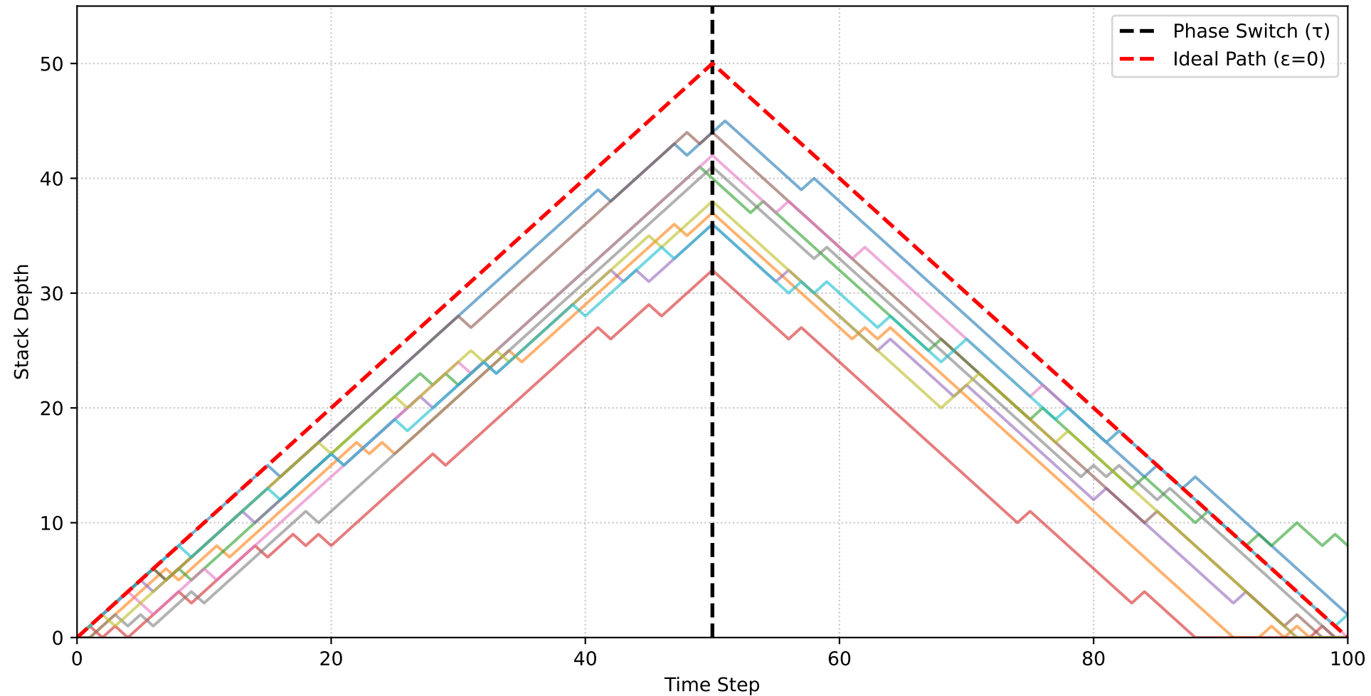
Soft Stack Depth Random Walks ( N=50 , \varepsilon=0.1 )
