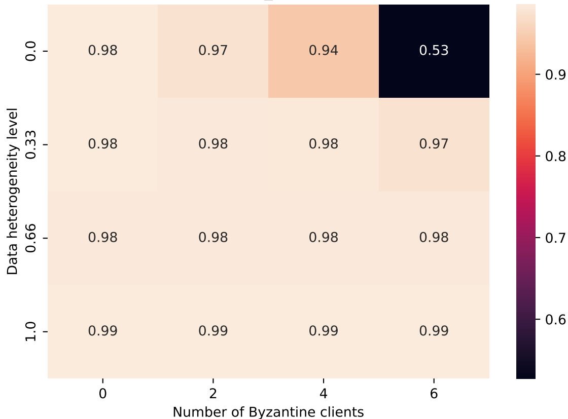
Attack: Optimal_ALittleIsEnough
