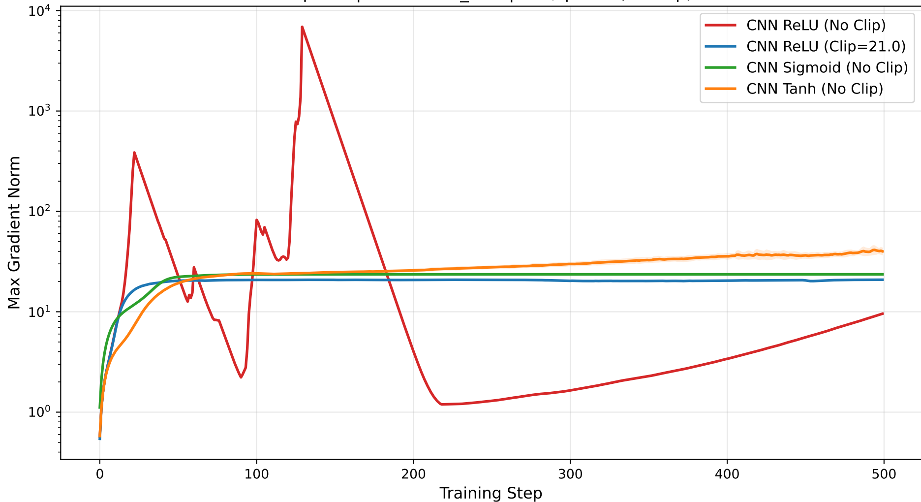
Max Gradient Norm OptIPM | GM + NNM_ARC | f=1 , \gamma=0.0 (No Clip)
