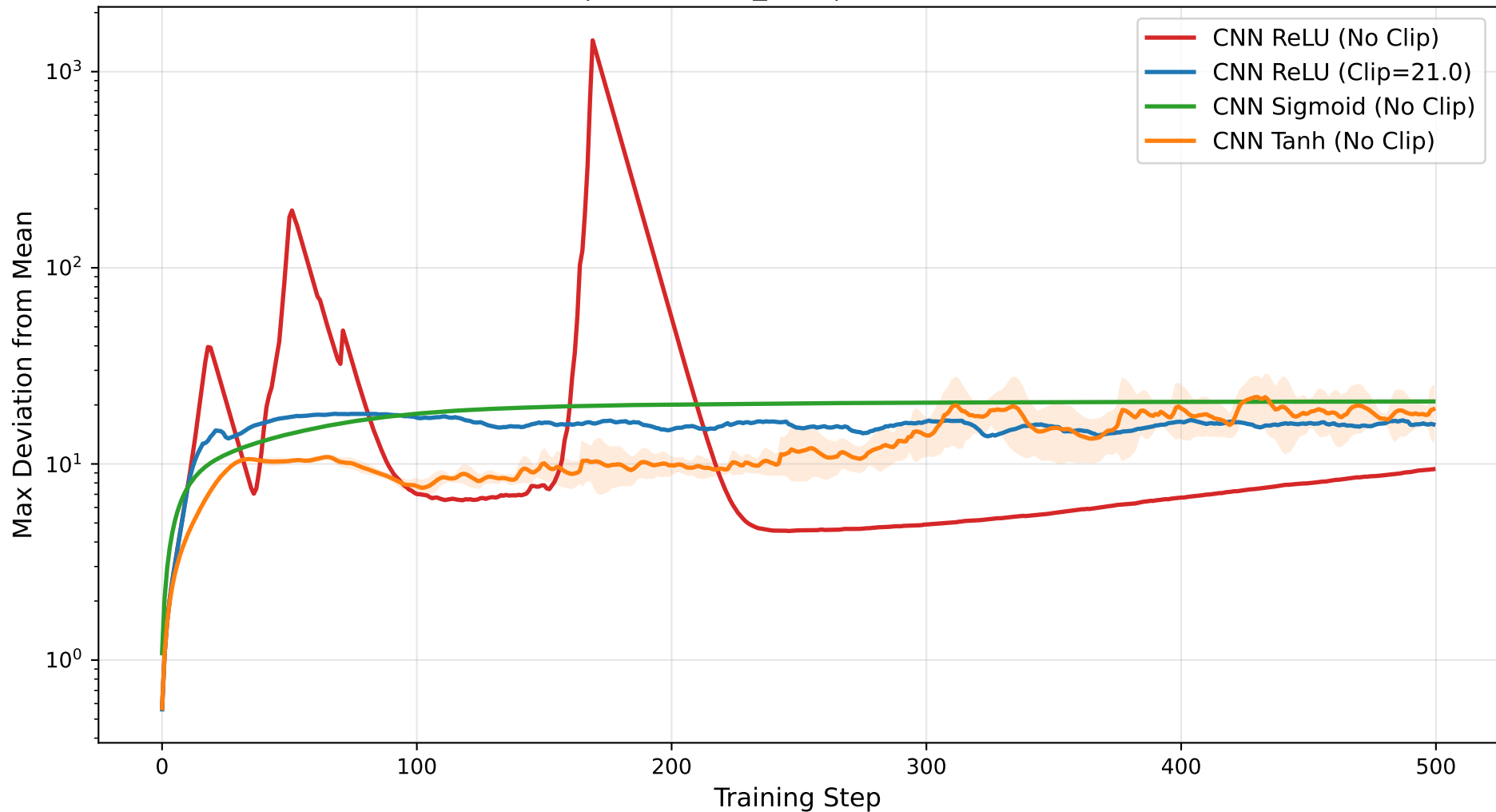
Max Deviation from Mean OptALIE | GM + NNM_ARC | f=1 , \gamma=0.0 (No Clip)
