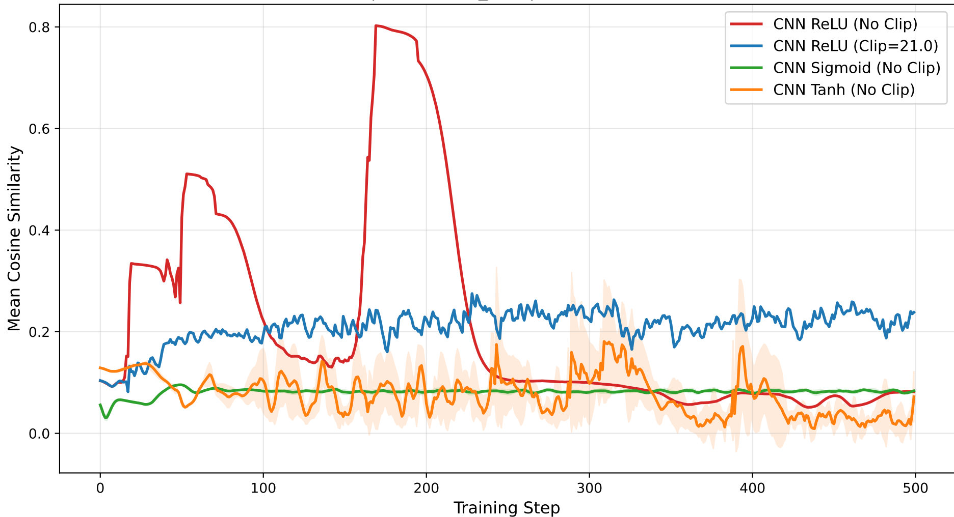
Mean Cosine Similarity OptALIE | GM + NNM_ARC | f=1 , \gamma=0.0 (No Clip)
