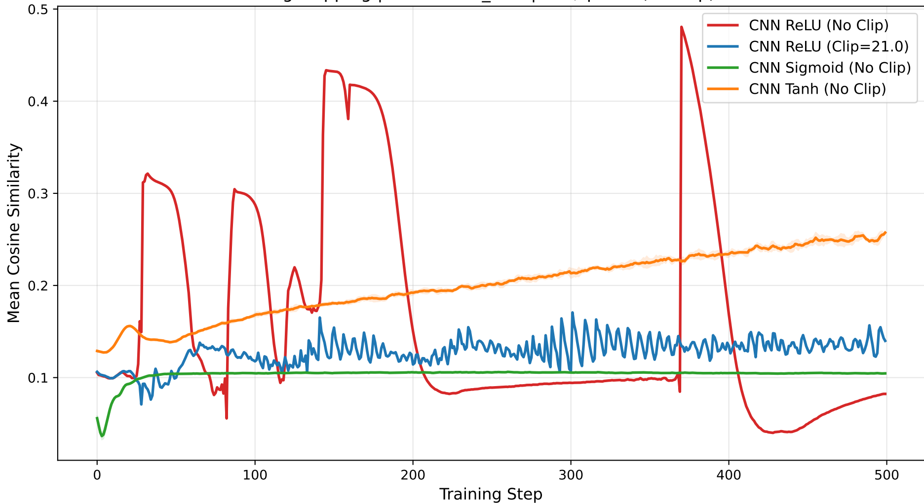
Mean Cosine Similarity SignFlipping | GM + NNM_ARC | f=1 , \gamma=0.0 (No Clip)
