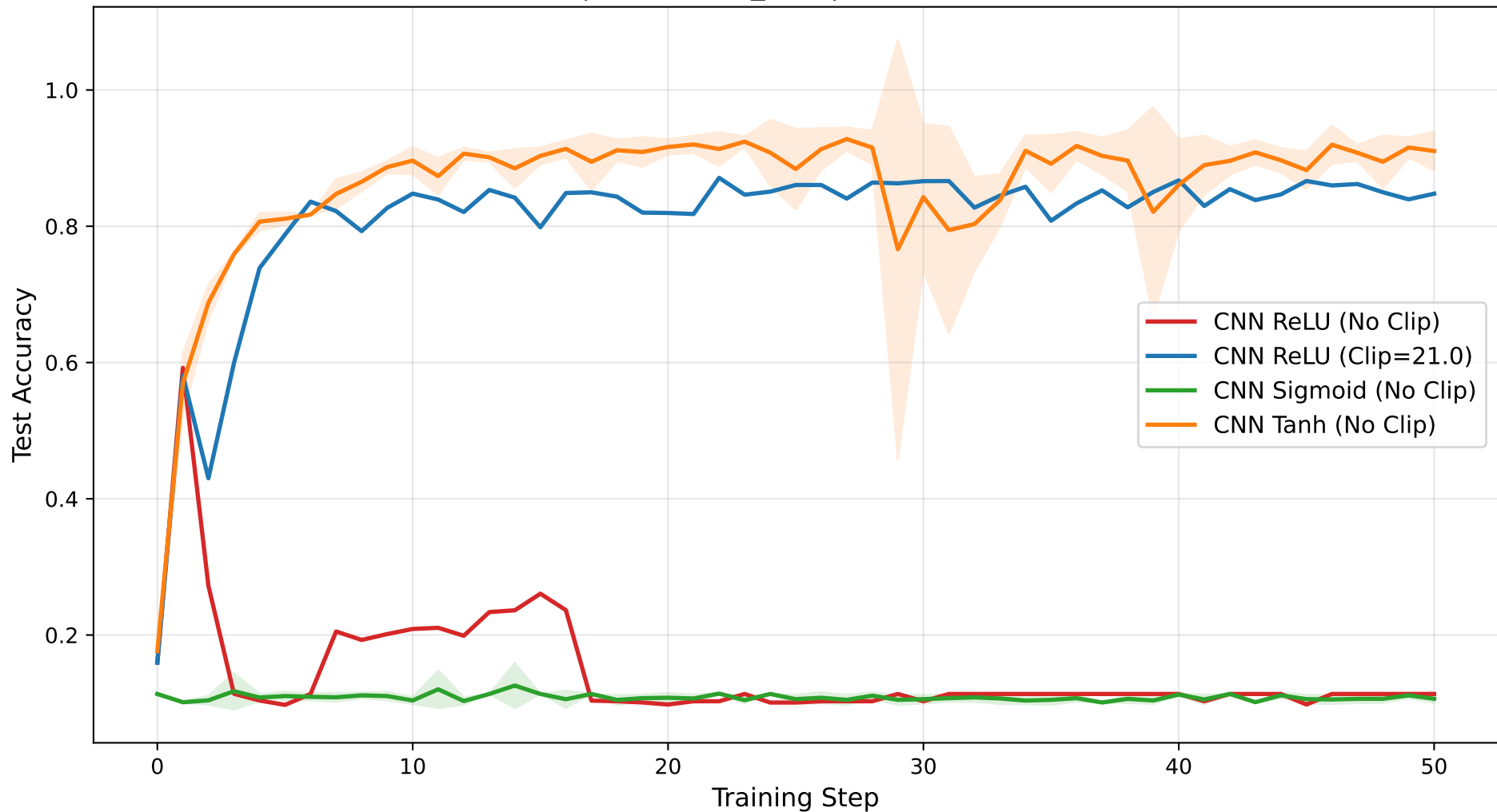
Test Accuracy OptALIE | GM + NNM_ARC | f=1 , \gamma=0.0 (No Clip)
