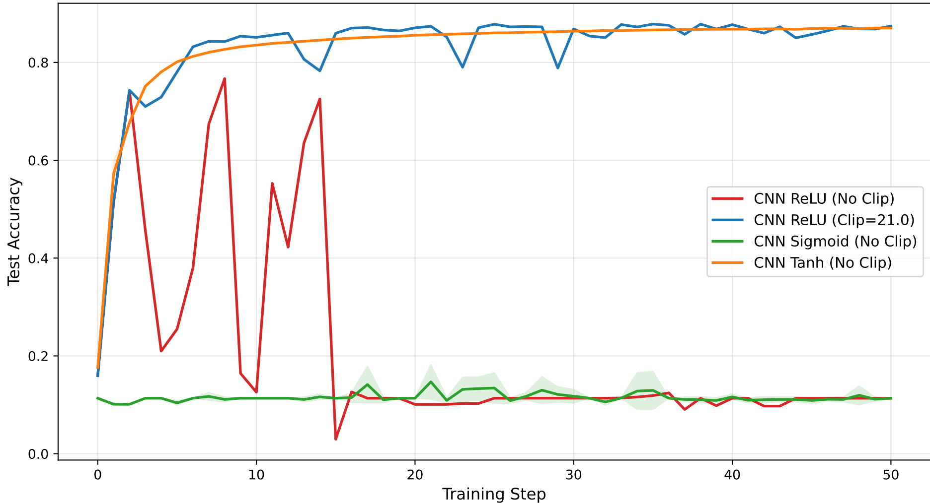
Test Accuracy SignFlipping | GM + NNM_ARC | f=1 , \gamma=0.0 (No Clip)
