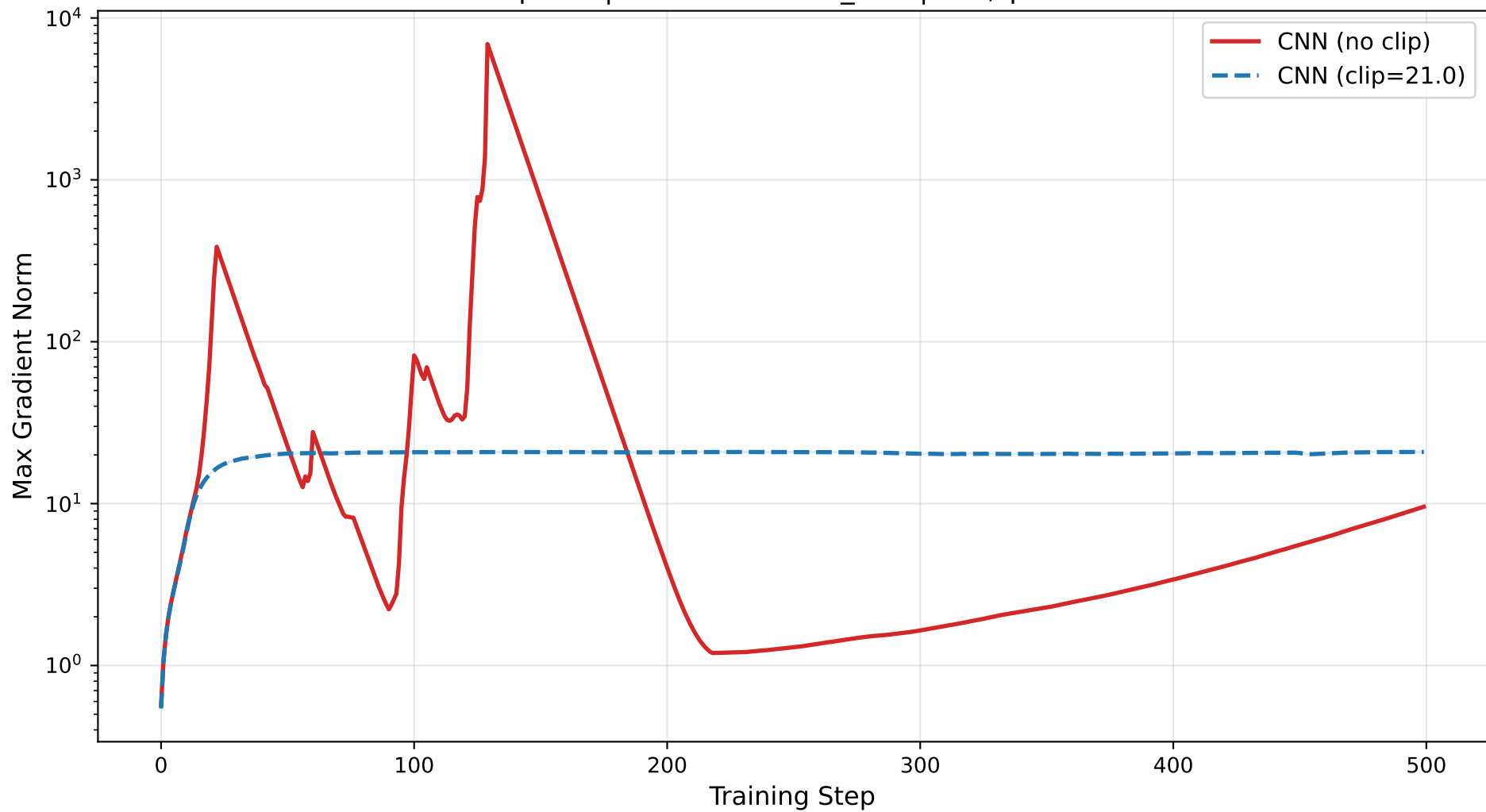
Max Gradient Norm OptIPM | GeoMed + NNM_ARC | f=1 , \gamma=0.0
