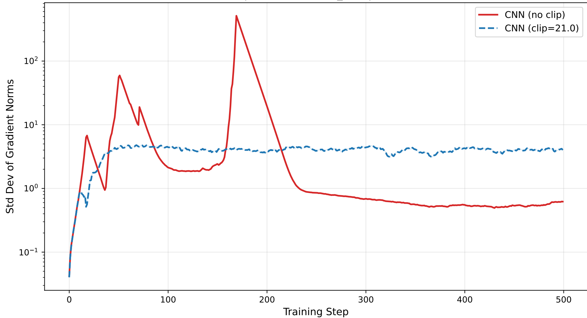
Std Dev of Gradient Norms OptALIE | GeoMed + NNM_ARC | f=1 , \gamma=0.0
