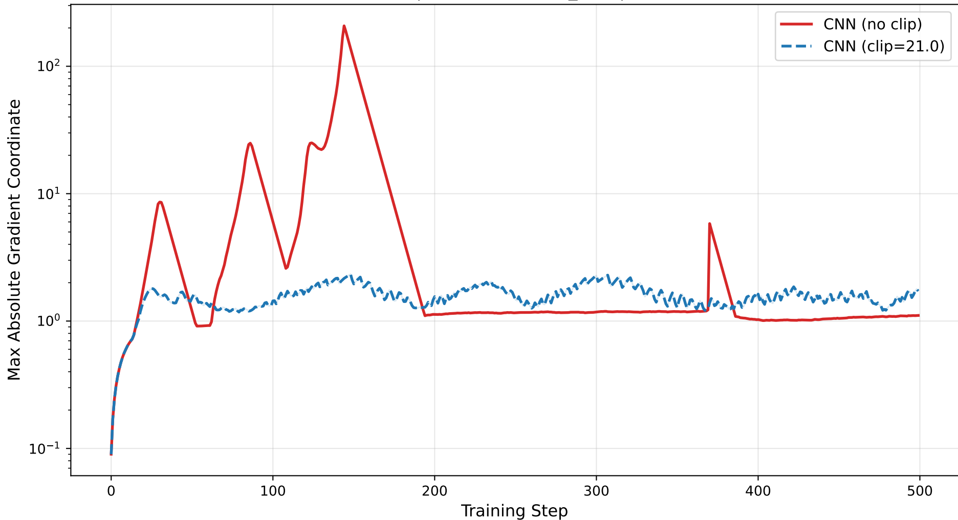
Max Absolute Gradient Coordinate SignFlipping | GeoMed + NNM_ARC | f=1 , \gamma=0.0
