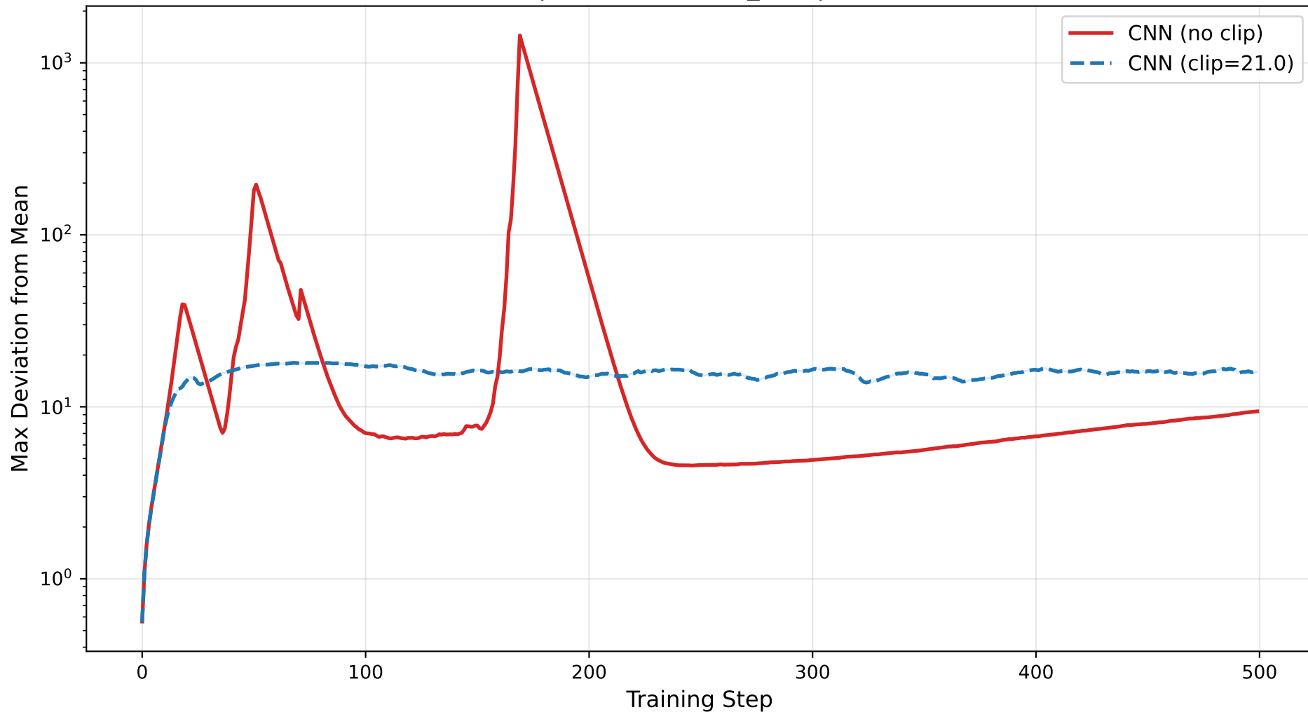
Max Deviation from Mean OptALIE | GeoMed + NNM_ARC | f=1 , \gamma=0.0
