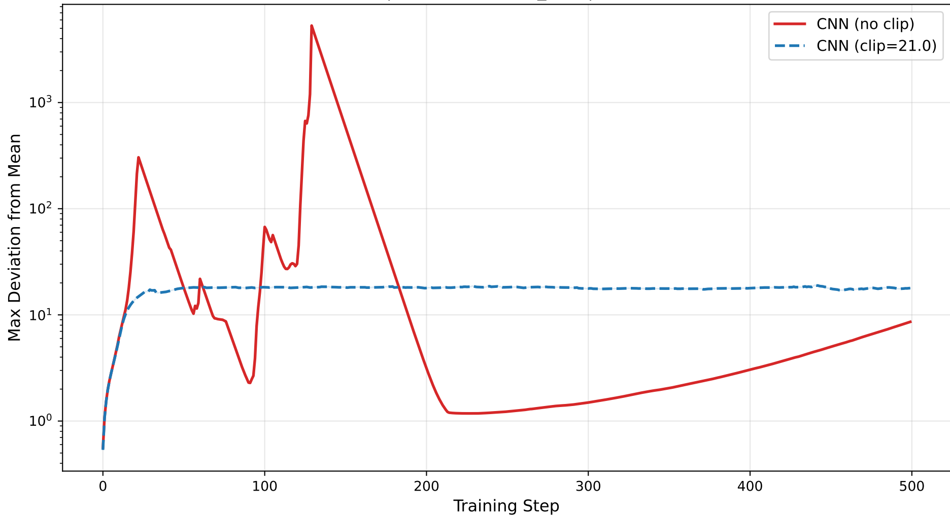
Max Deviation from Mean OptIPM | GeoMed + NNM_ARC | f=1 , \gamma=0.0
