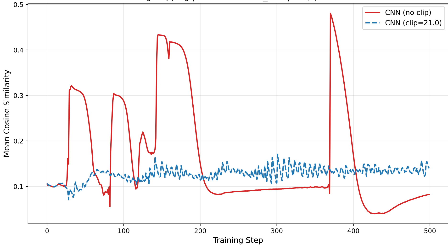
Mean Cosine Similarity SignFlipping | GeoMed + NNM_ARC | f=1 , \gamma=0.0
