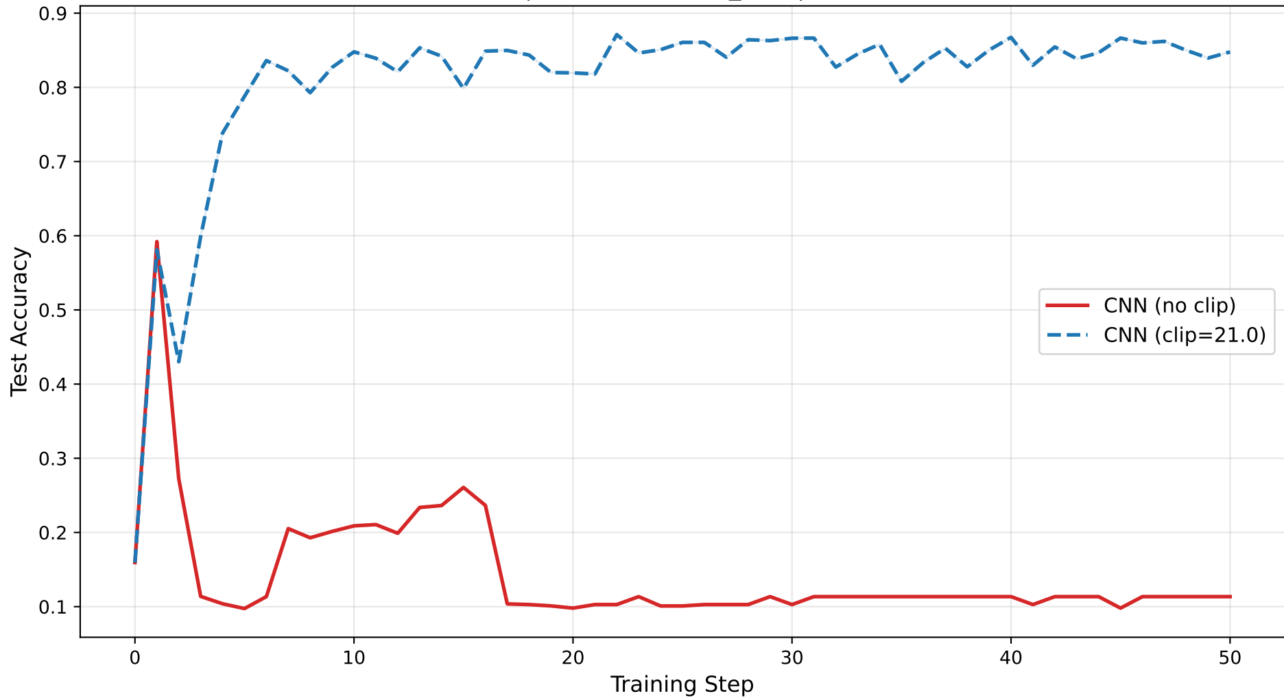
Test Accuracy OptALIE | GeoMed + NNM_ARC | f=1 , \gamma=0.0
