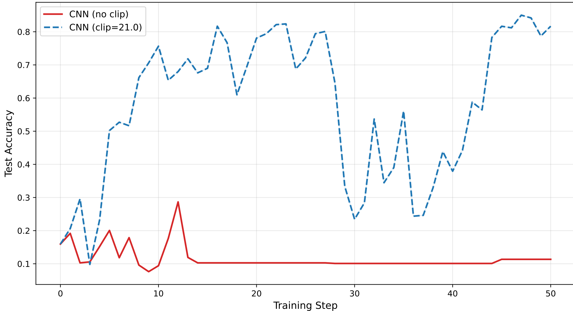
Test Accuracy OptIPM | GeoMed + NNM_ARC | f=1, \gamma=0.0
