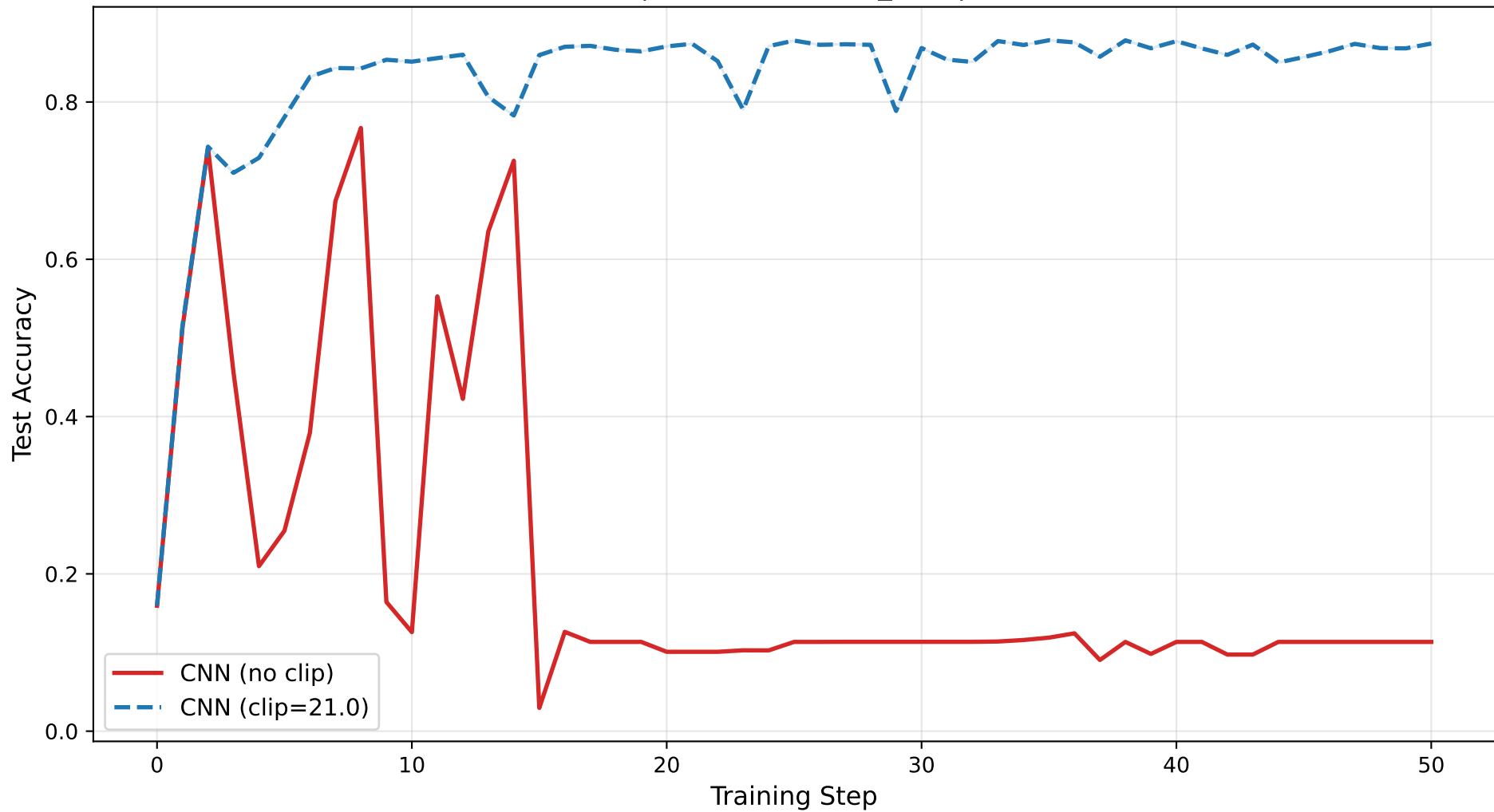
Test Accuracy SignFlipping | GeoMed + NNM_ARC | f=1, \gamma=0.0
