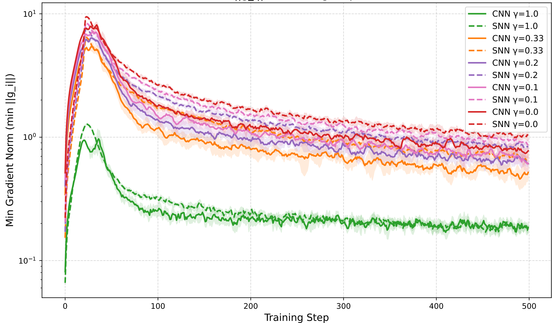
Min Gradient Norm (min \|g_i\| ) vs Training Step (CNN solid, SNN dashed)
