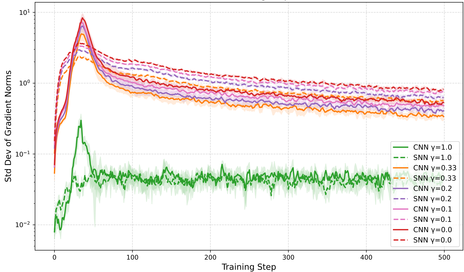
Std Dev of Gradient Norms vs Training Step (CNN solid, SNN dashed)
