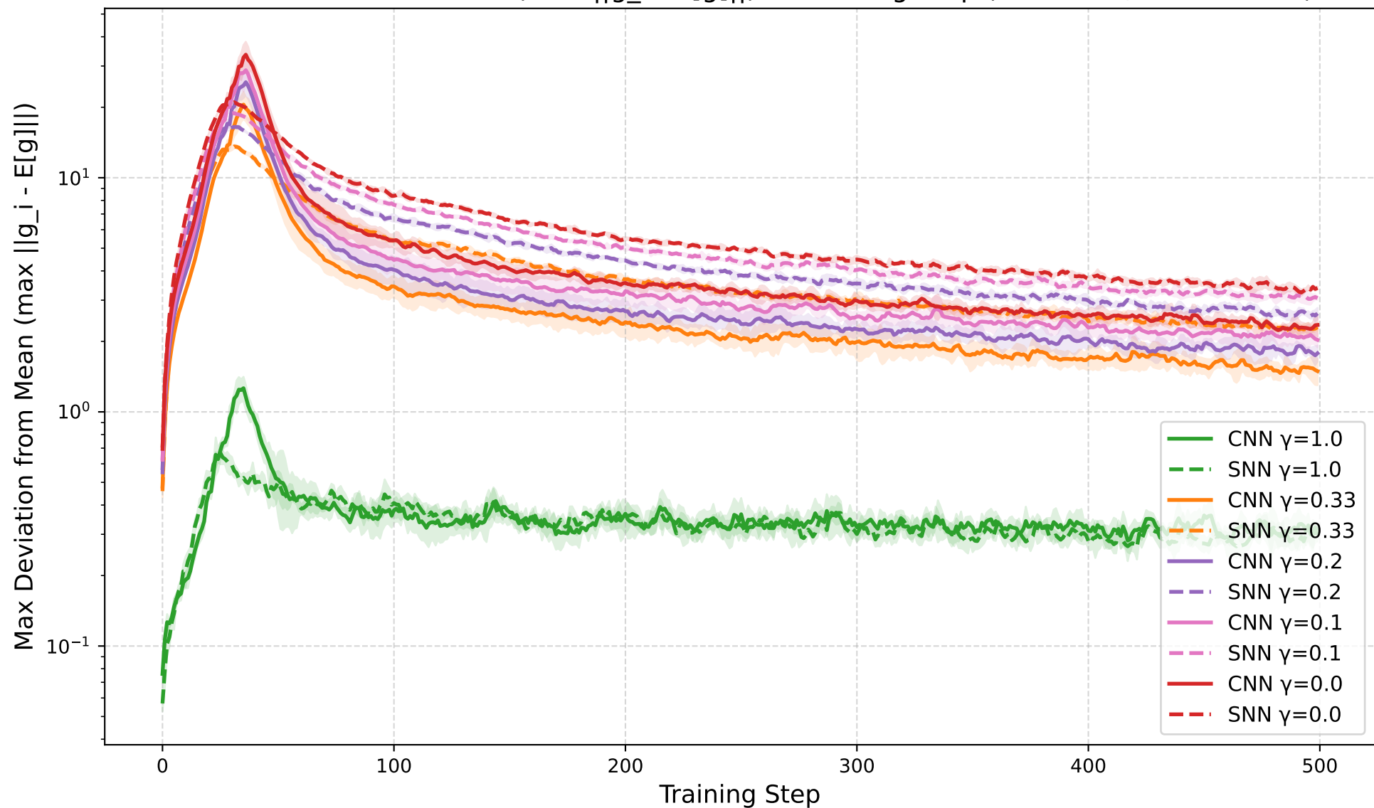
Max Deviation from Mean ( \max ||g_i - E[g]|| ) vs Training Step (CNN solid, SNN dashed)
