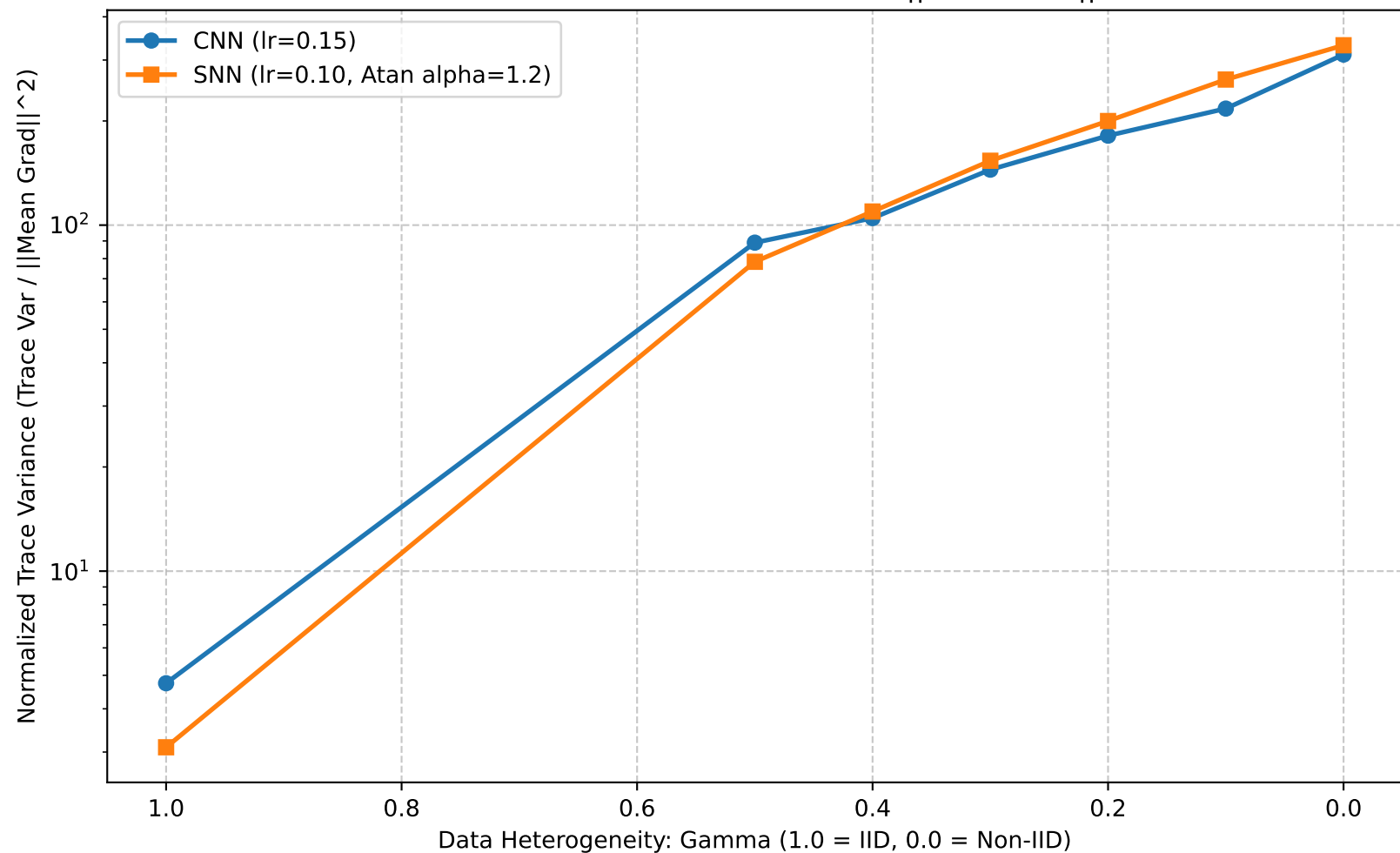
Normalized Trace Variance (Trace Var / \|\text{Mean Grad}\|^2 )
