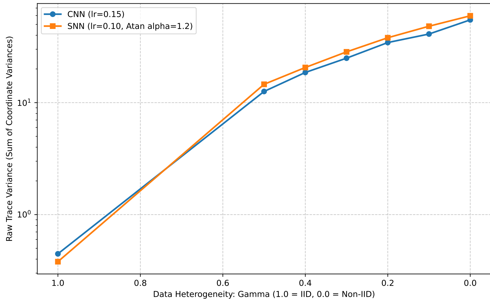
Raw Trace Variance (Sum of Coordinate Variances)
