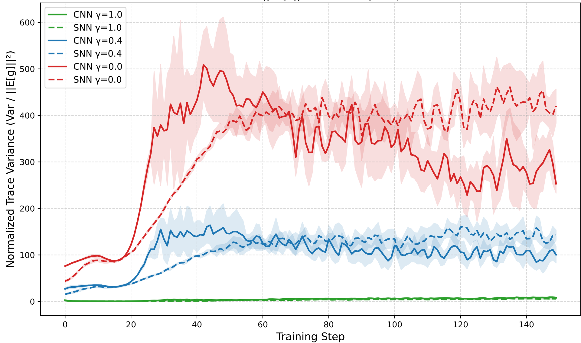
Normalized Trace Variance ( \text{Var} / ||E[g]||^2 ) vs Training Step (CNN solid, SNN dashed)
